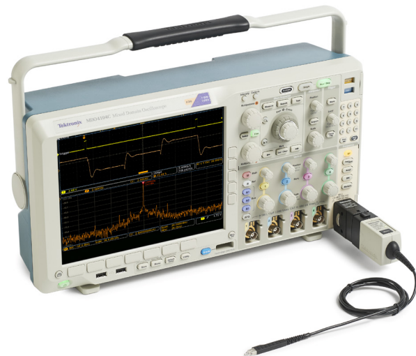
The optional TPA-N-VPI adapter enables any active, 50 \Omega TekVPI probe to be connected to the RF input.
